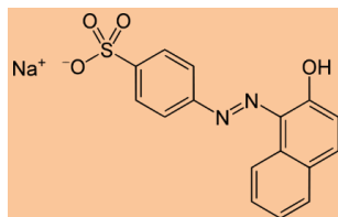
Sodium 4-[(2E)-2-(2-oxonaphthalen-1-ylidene)hydrazinyl]benzenesulfonate
