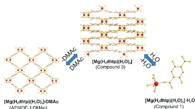
Fig. 5 Structural transformations observed for compound 3 .
