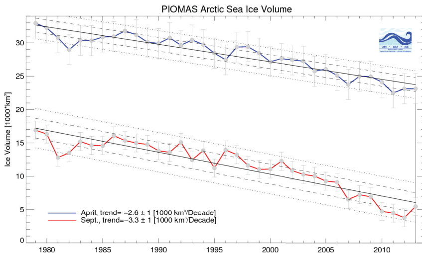
Figure 1: PIOMAS Arctic Sea Ice Volume
