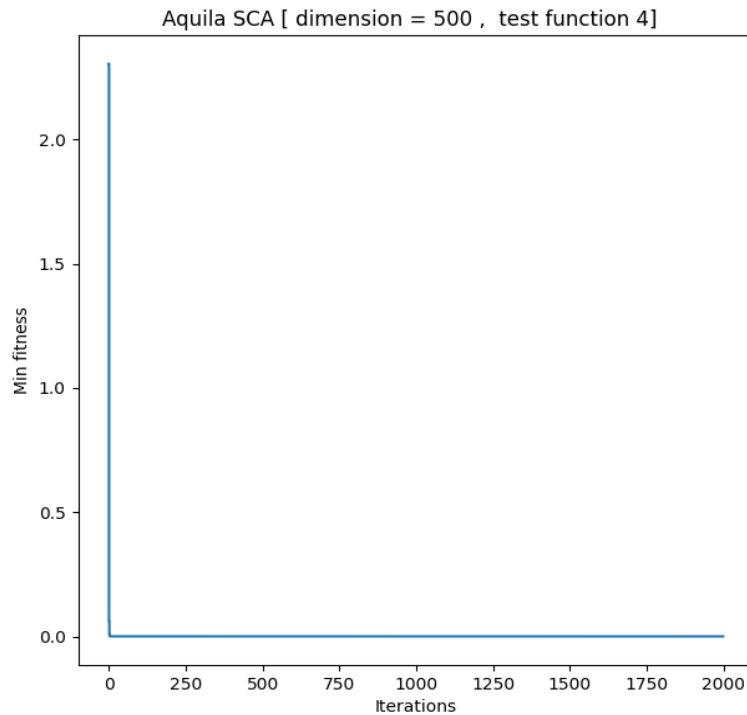
Figure 16: Aquila’s Min Fitness/iteration diagram (dimension=500)
