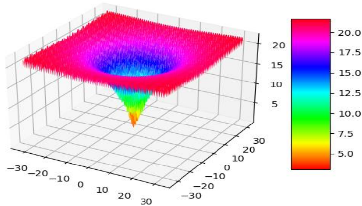
Figure 10:Ackley 3-dimension graph
