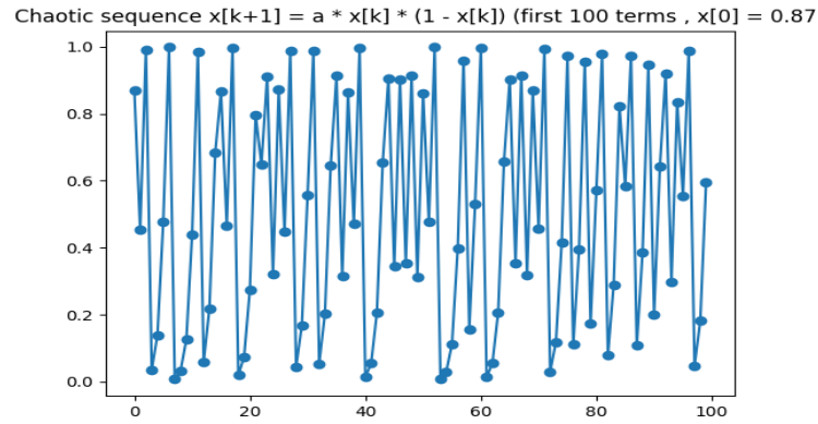
Figure 5: Logistic map (first 100 terms)
