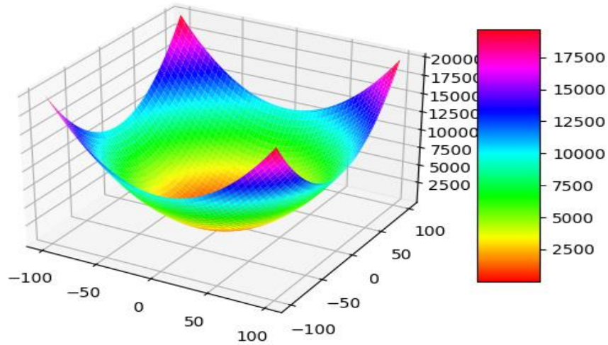
Figure 8: Schwefel's seven 3-dimension graph
