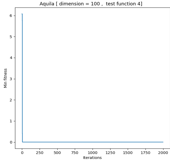
Figure 13: Aquila's Min Fitness/iteration diagram (dimension=100)
