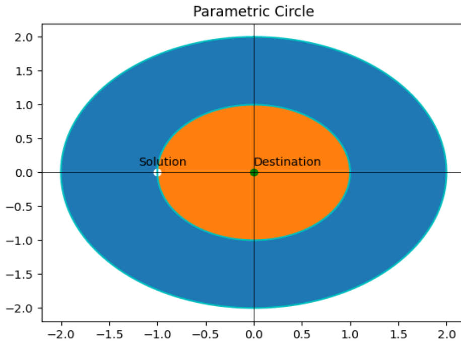
Figure 1: Approximation of solution depending on the destination radius.
