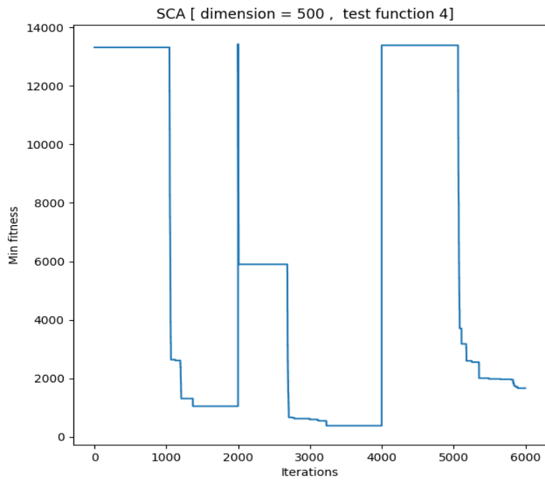
Figure 14: Basic SCA's Min Fitness/iteration diagram (dimension=500)
