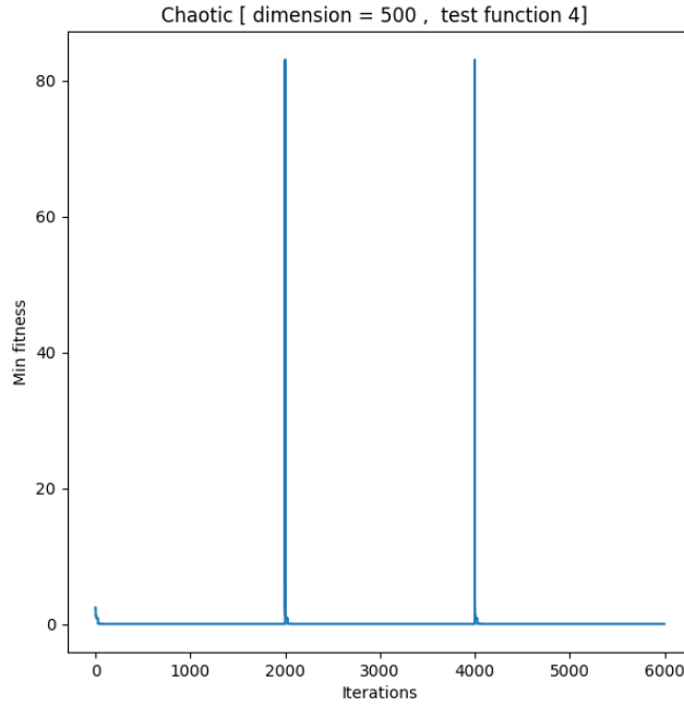
Figure 15: Chaotic SCA’s Min Fitness/iteration diagram (dimension=500)
