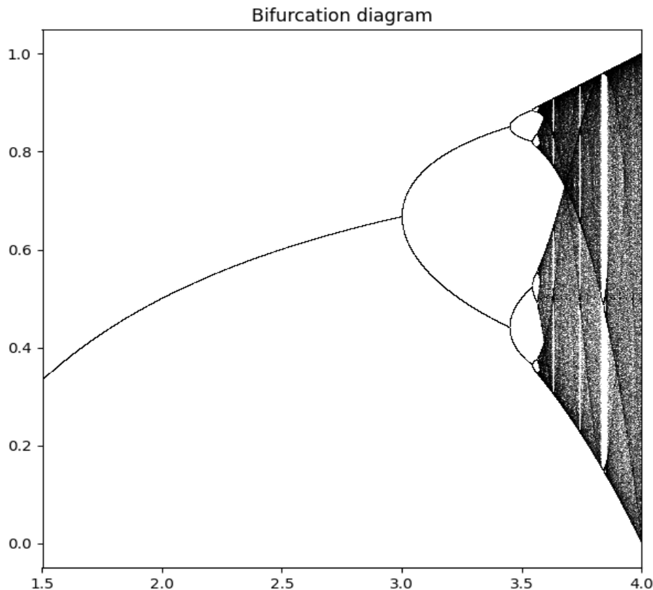
Figure 4: Bifurcation diagram
