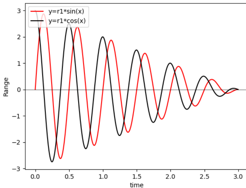
Figure 3: Decreasing amplitude of the trigonometric functions
