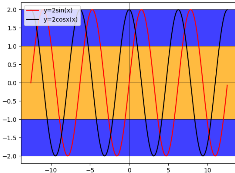
Figure 2: Decision of radius based on values of Sine and Cosine
