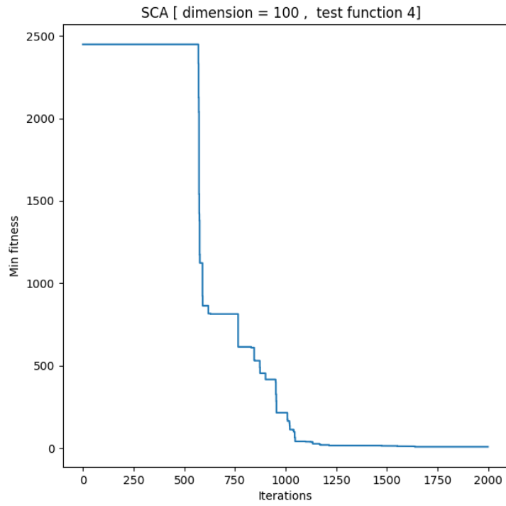
Figure 11: Basic SCA's Min Fitness/iteration diagram (dimension=100)
