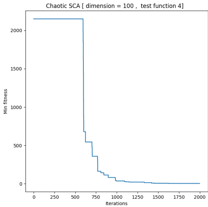
Figure 12: Chaotic SCA's Min Fitness/iteration diagram (dimension=100)
